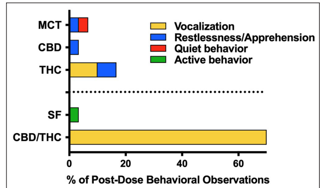
Figure 6 Proportion and profile of behavioral observations attributed to dose escalation of cannabis or placebo oils ( n = 4 per treatment) that were observed within 24 h of oil administration across 11 escalating doses. Restlessness/apprehension includes observations of fractious behavior, pacing, agitation and/or nervousness. MCT = medium-chain triglyceride oil; CBD = cannabidiol; THC = tetrahydrocannabinol; SF = sunflower oil
